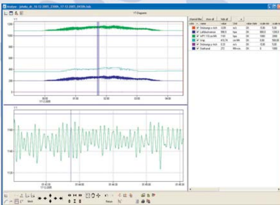
Measuring wave surges at a dike
