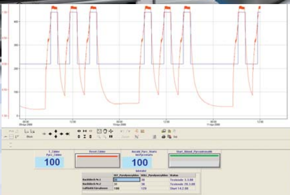
Automated endurance testing at an oven test stand
